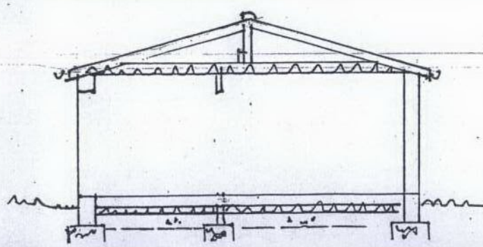
Proposed Extensions at N° 97 Perne Road, Cambridge - Section AA @ 1:100 scale.
