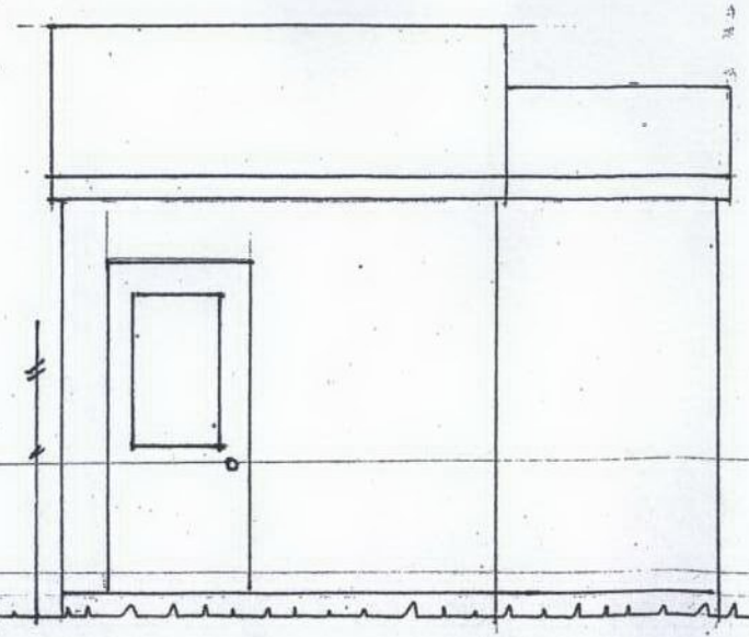
Proposed Extensions at N° 97 Perne Road, Cambridge - Section AA @ 1:100 scale.
